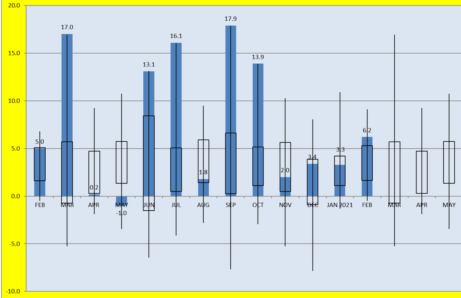
Control State 9L Cases % Chg over Same Month Last Year Through February, 2021 with Monthly Avg High and Low, as well as All-Time High and Low, Growth Rates
