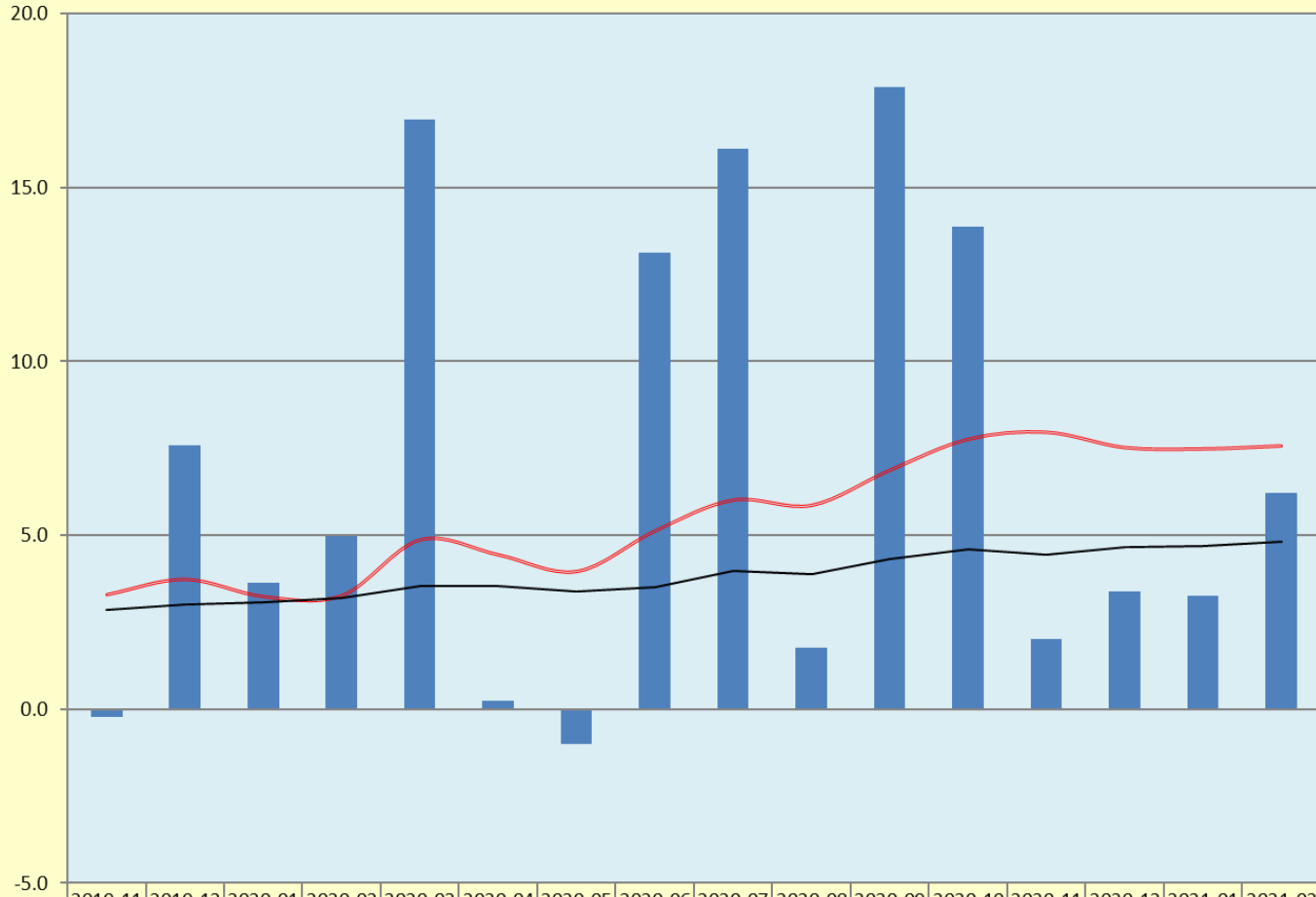
9 Liter Case Spirits Growth in the Control States as of February, 2021: Month over Same Month Last Year % Change, Rolling-12 Month % Change, and 3 Year CAGR
