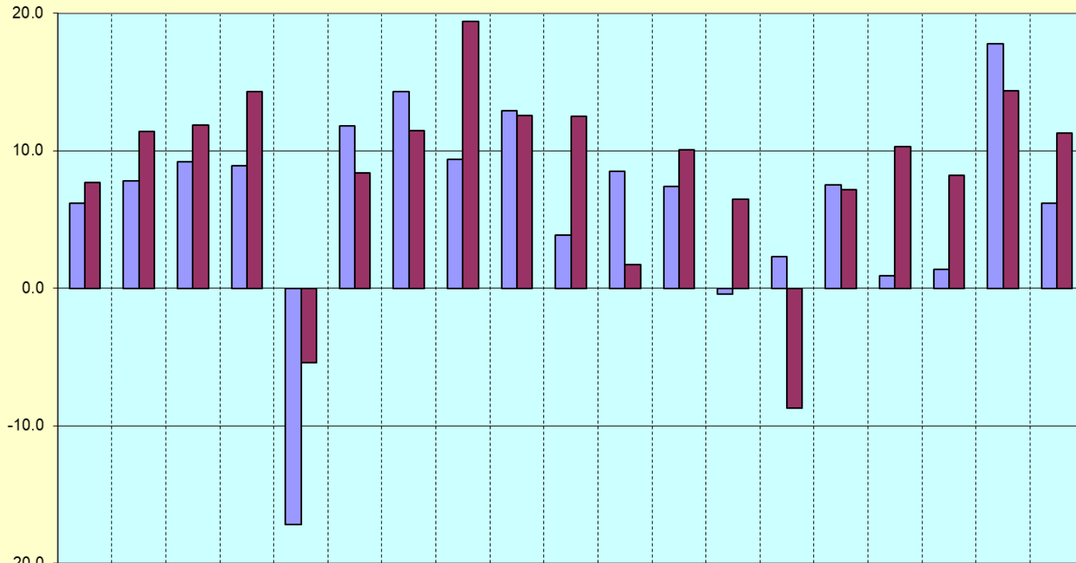
Nine Liter Case Spirits Growth in the Control States by State for February, 2021: Month over Same Month Last Year % Change and Rolling-12-Month % Change
